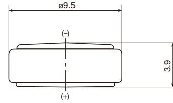
Unit: mm
