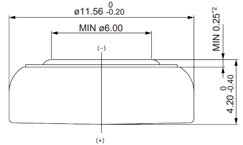
*2 The dimension is measured from the top surface of the negative can.
